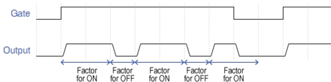
Behaviour of Continuous Pulse Generator
