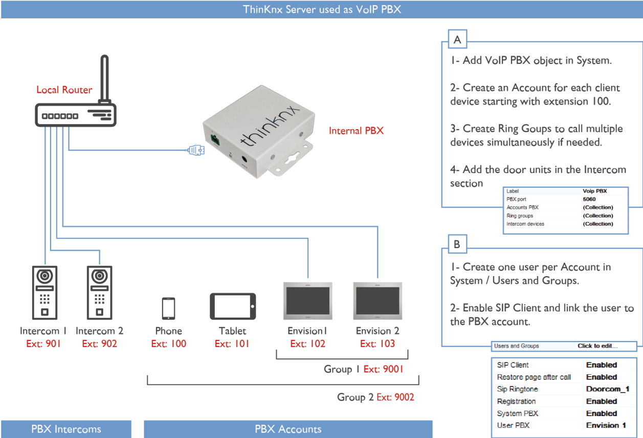
Thinknx server used as a VoIP PBX
