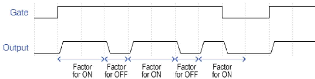
Behaviour of Continuous Pulse Generator
