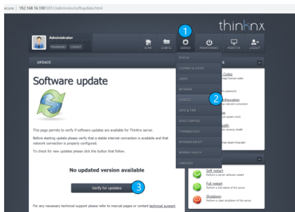
Figure 3.4: Server Update
