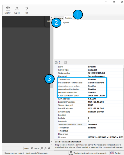
Figure 5.2.2.1: Configuring Cloud inside Configurator
